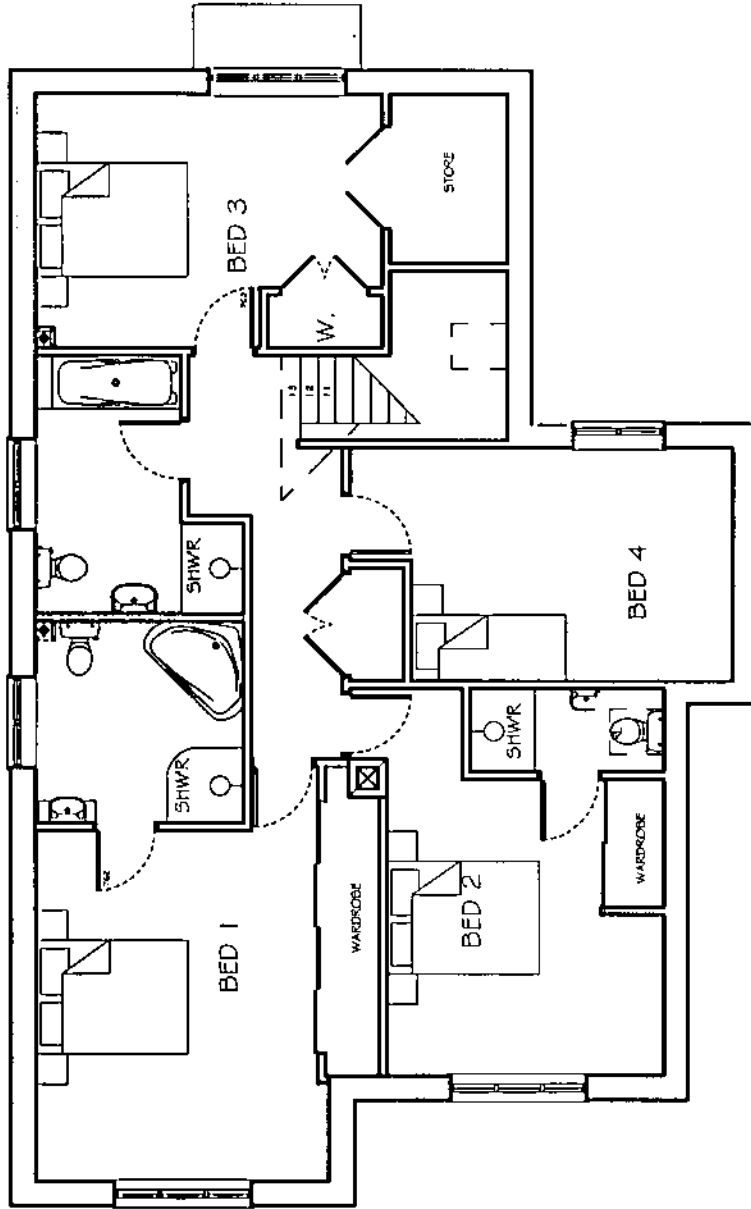
FIRST FLOOR PLAN 106 SQM
